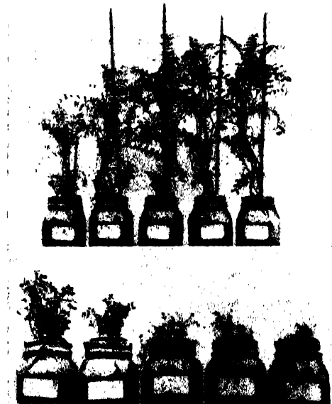
OPPOSITE EFFECTS OF SELENIUM ON TWO SPECIES OF Astragalus . Above: Astragalus racemosus STIMULATED BY SELENIUM. Below: Astragalus crassicaarpus POISONED BY SELENIUM. SELENIUM CONCENTRATIONS IN CULTURE SOLUTIONS (left to right): 0, \frac{1}{2} , 1, 3, 9 PARTS PER MILLION.
